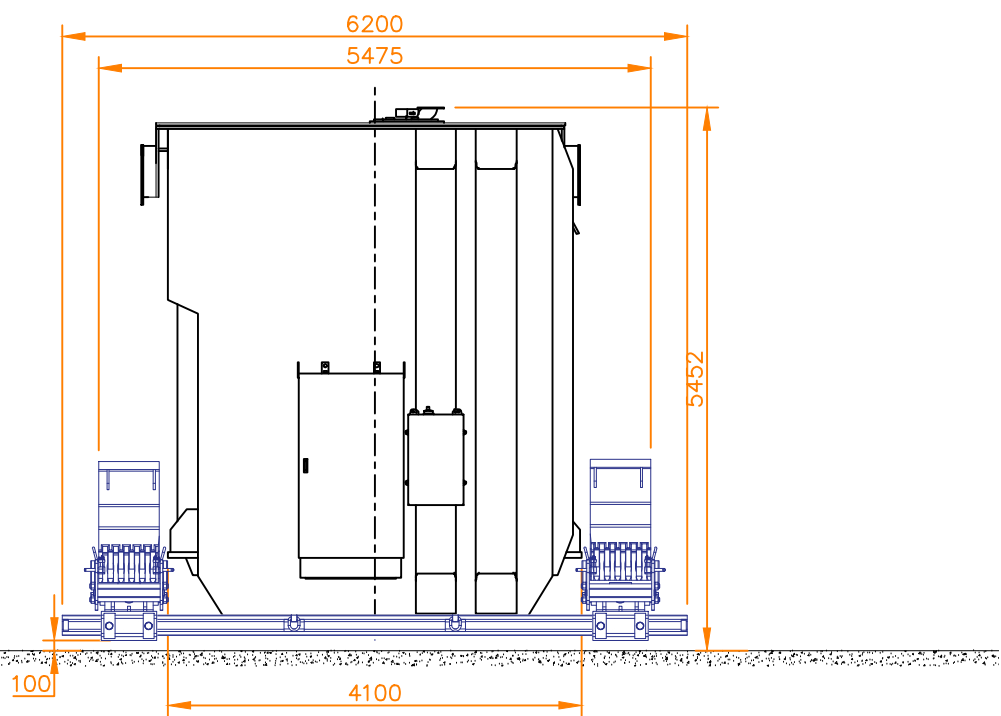
TRAF0 ON BEAMS REAR ELEVATION VIEW. SCALE 1:75
